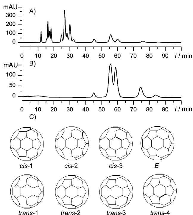
Figure 1. HPLC chromatograms of the mixtures of isomers of bis-PCBM obtained by standard bis-addition (A) and from tethered addends (B) showing that less isomers are present in the latter. C) All possible regioisomers of bis-adducts of C_{60} .
