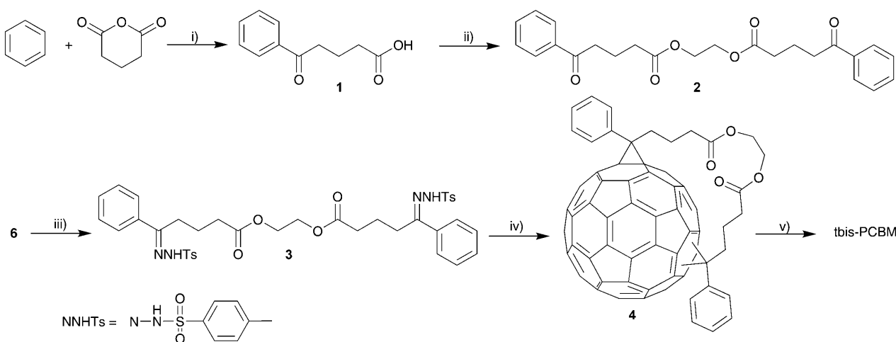
Scheme 1. Synthesis of the ethylene-tethered bis-(4-benzoylbutyric acid tosylhydrazone) 3 and the addition to the fullerene moiety. i) AlCl_3 , ClCH_2CH_2Cl ; ii) ethylene glycol, H^+ (cat.), toluene, Dean–Stark; iii) tosylhydrazide, toluene, Dean–Stark; iv) C_{60} , ODCB, t BuOK; v) MeOH, H^+ , ODCB.
