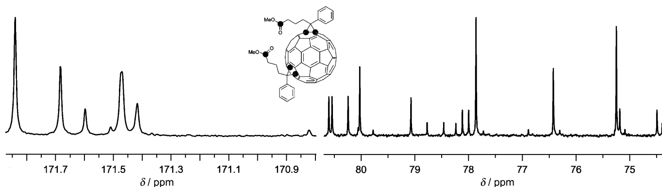
Figure 2. The ^{13}\text{C} NMR spectrum of the carbonyl (left) and bridgehead (right) area of the isomers obtained from tethered addends (a colour version of the figure is available in the Supporting Information).
